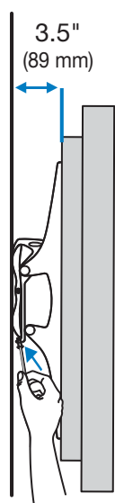
Wall Clearance
